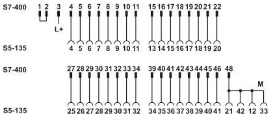
Connection diagram
