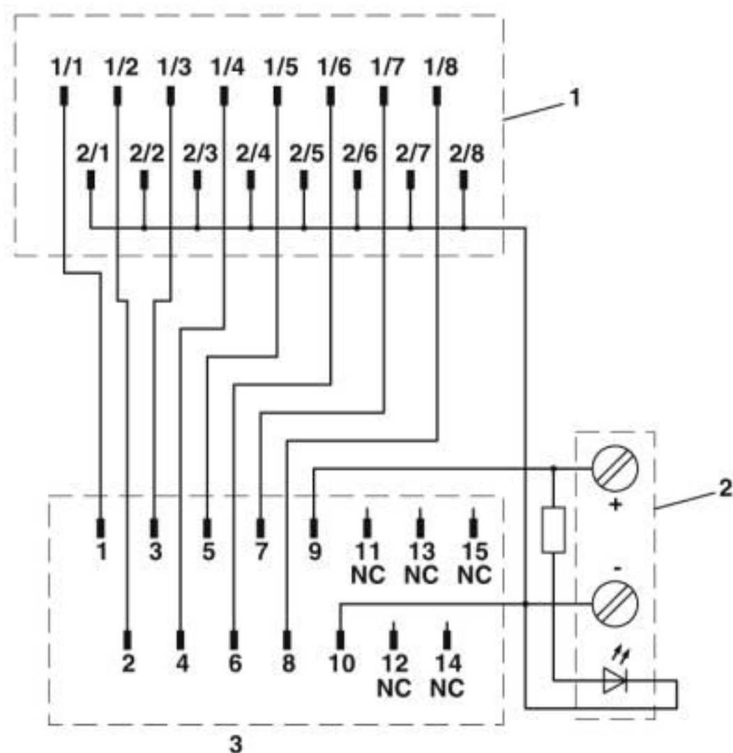
Circuit diagram
