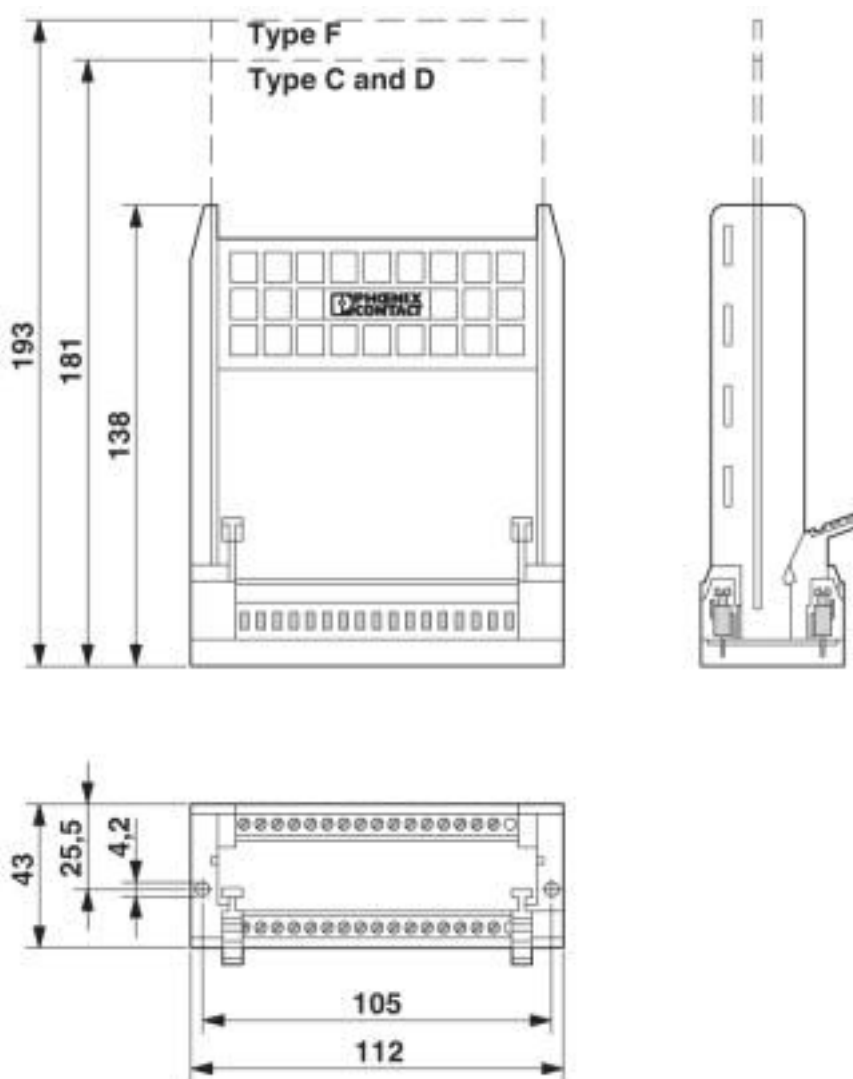
Dimensional drawing
