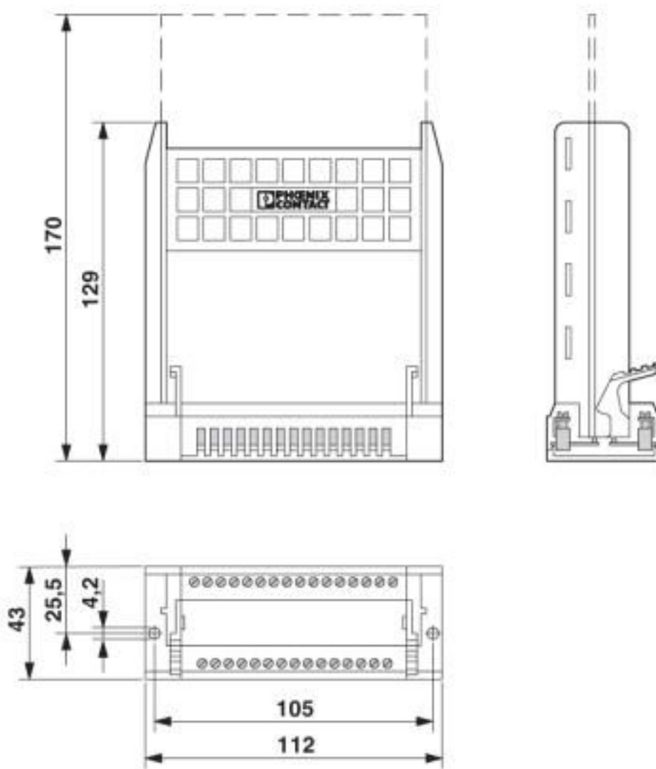
Dimensional drawing
