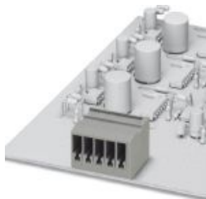
ST-COMBI receptacle, plug-in direction horizontal to the PCB, pitch: 5.2 mm, no. of positions: 5
