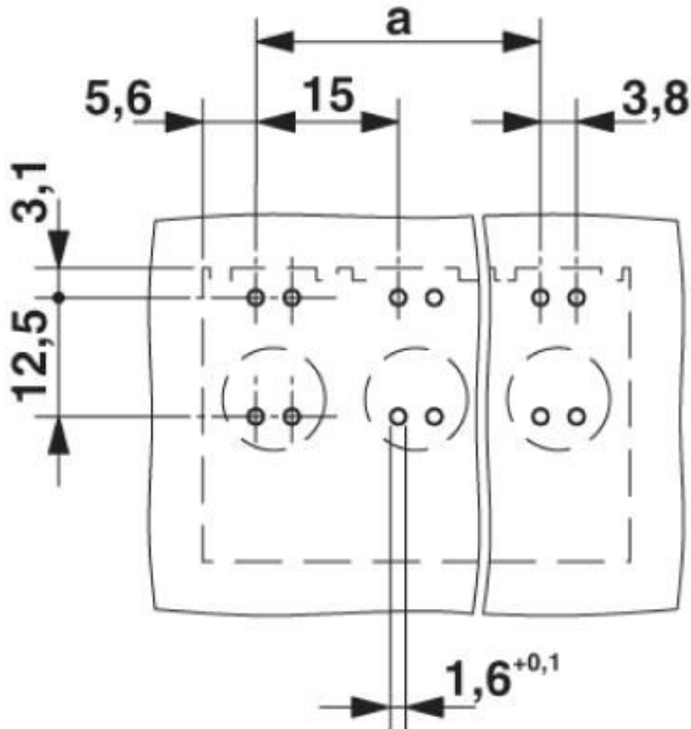
Drilling diagram
