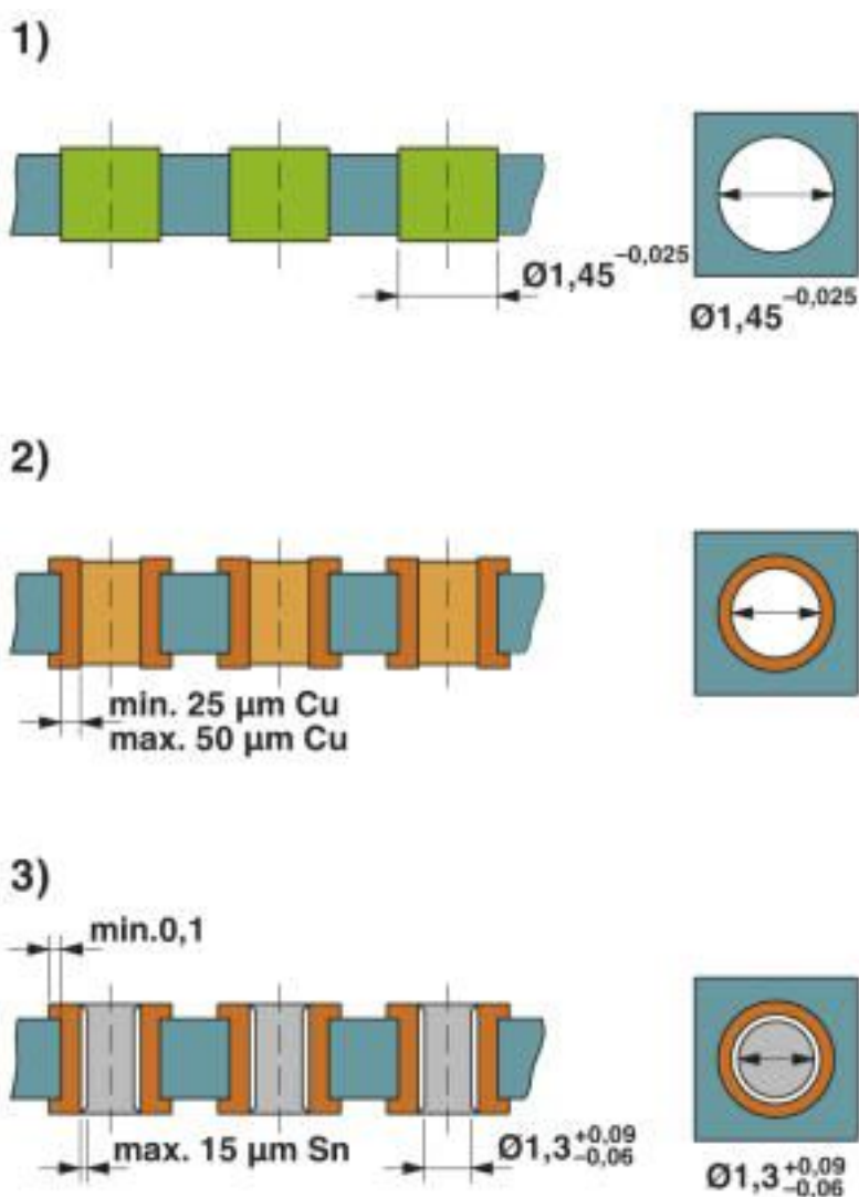
Drilling diagram
