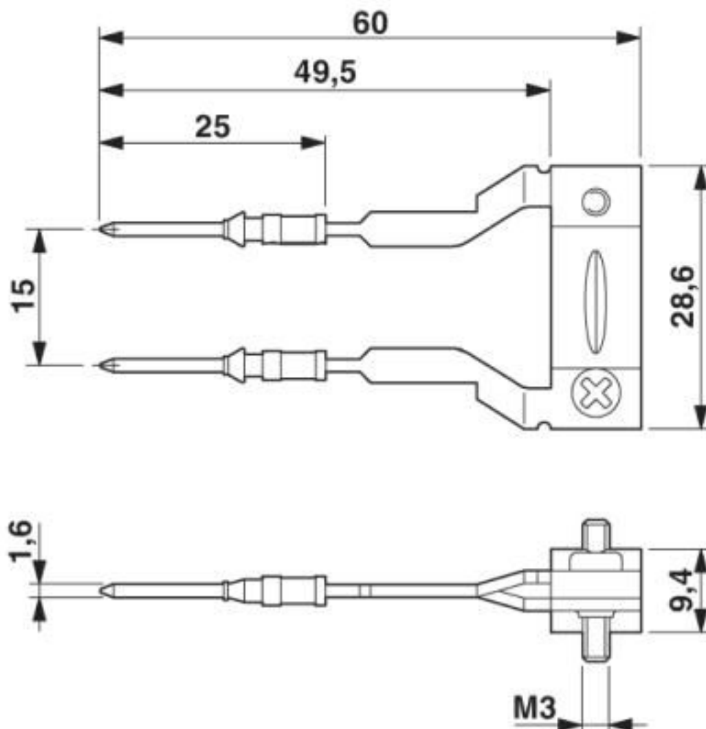
Dimensional drawing
