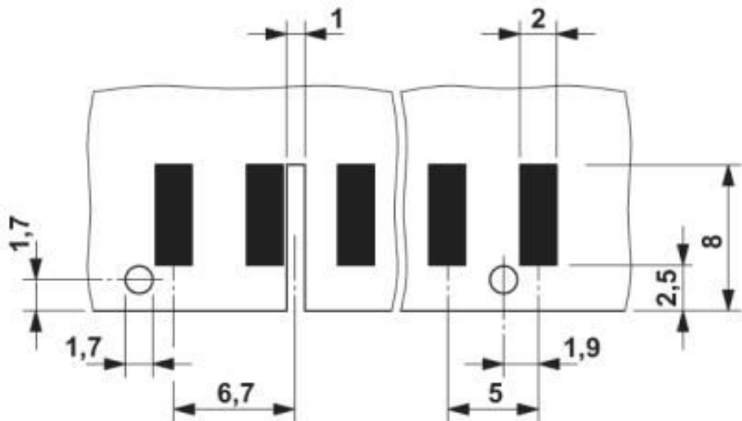
Drilling diagram
