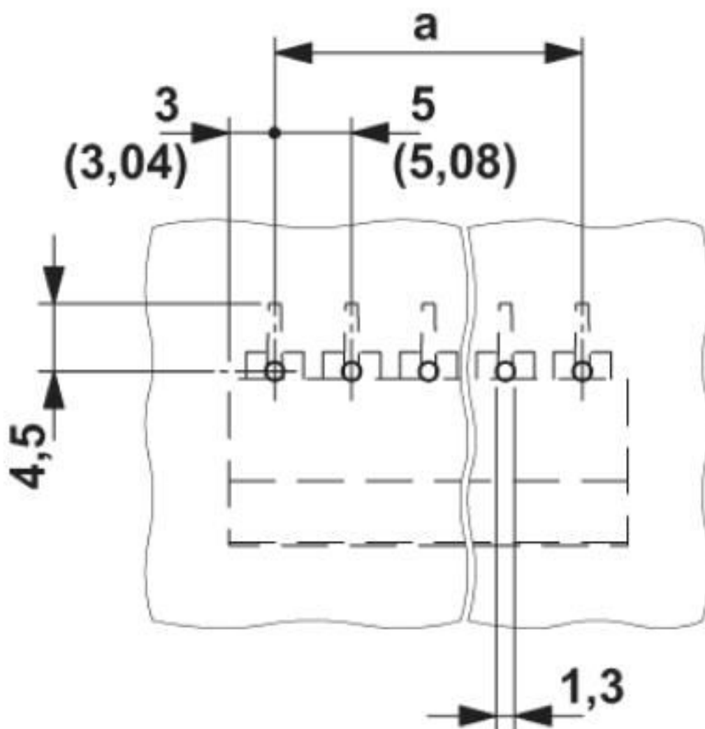
Drilling diagram
