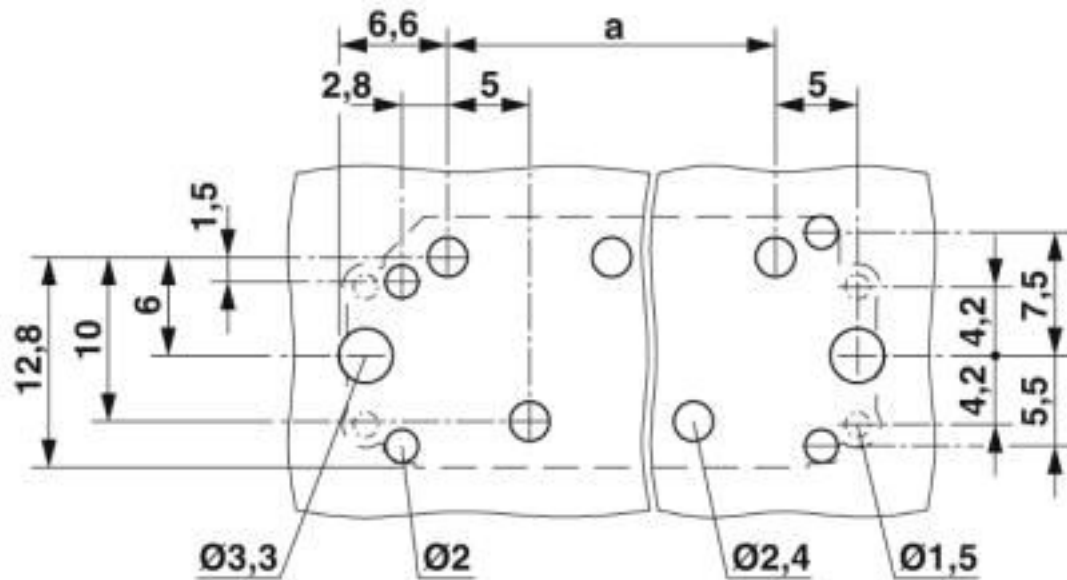
Drilling diagram
