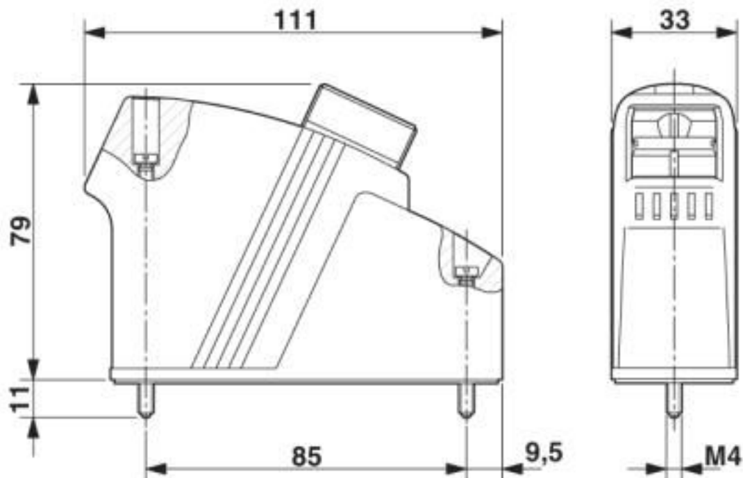
Dimensional drawing
