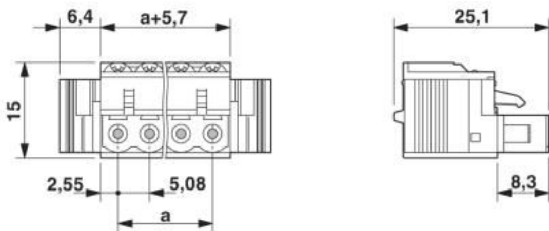
Dimensional drawing
