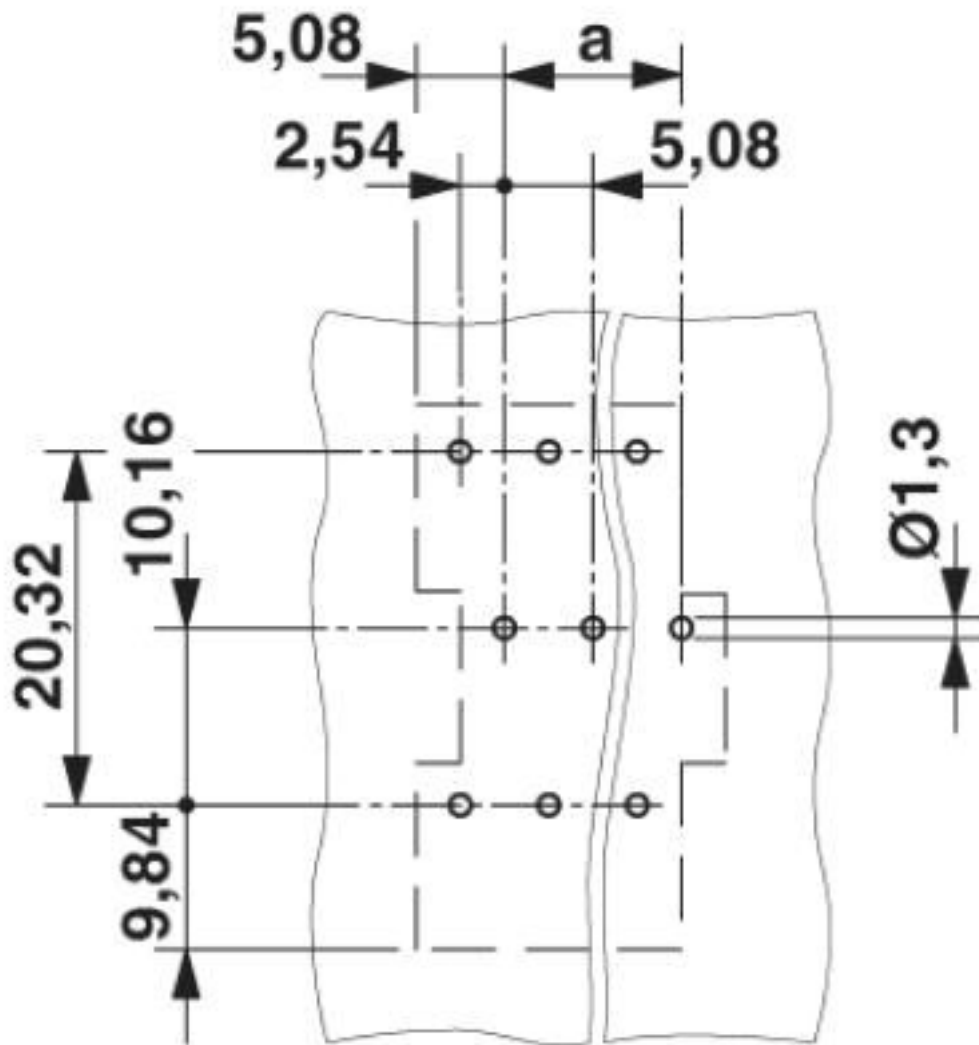
Drilling diagram
