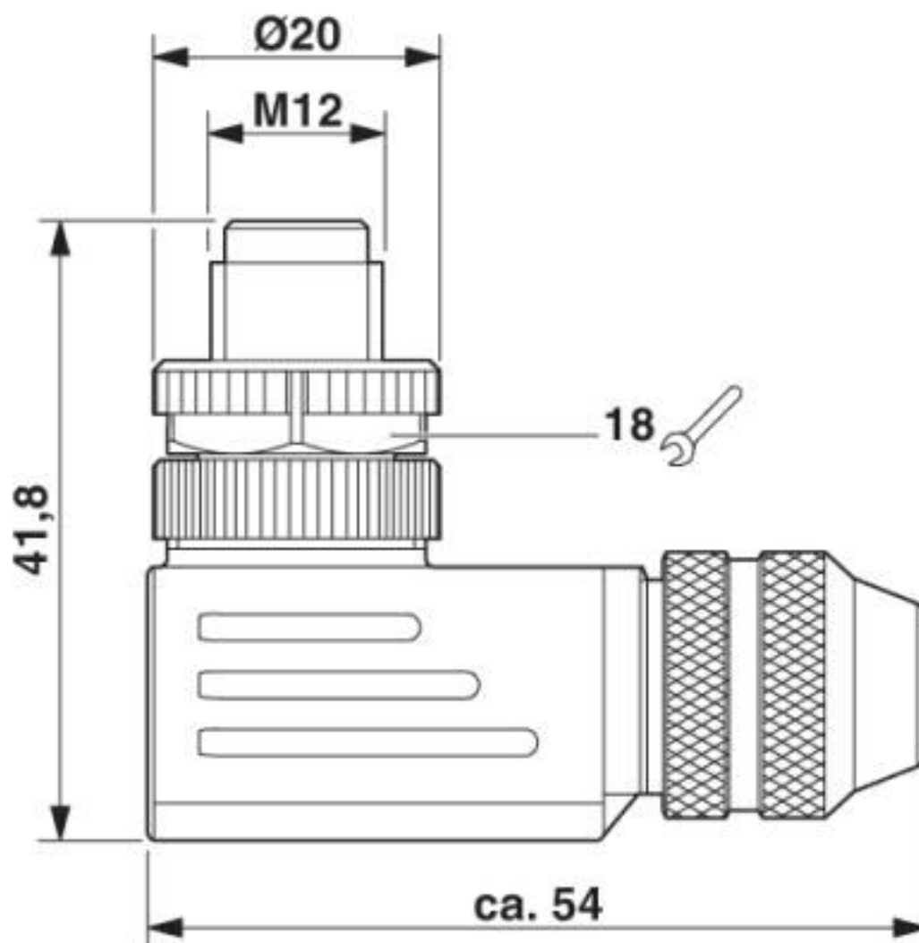
Dimensional drawing
