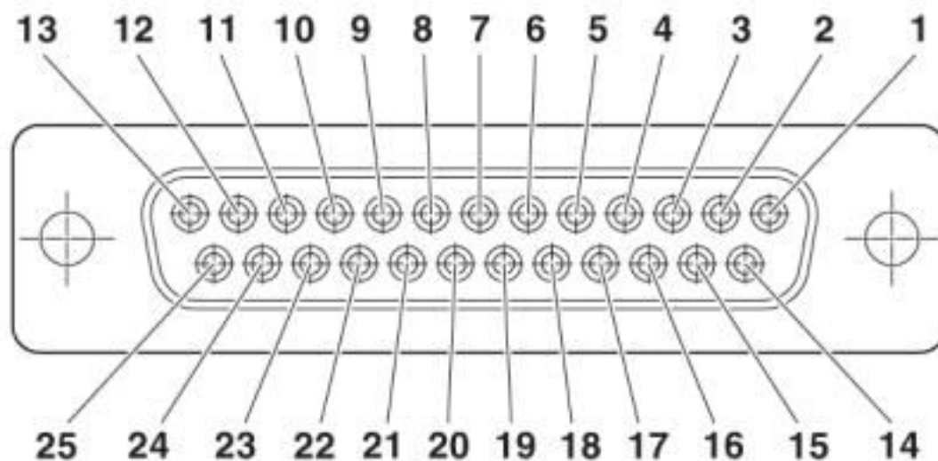
Schematic diagram
