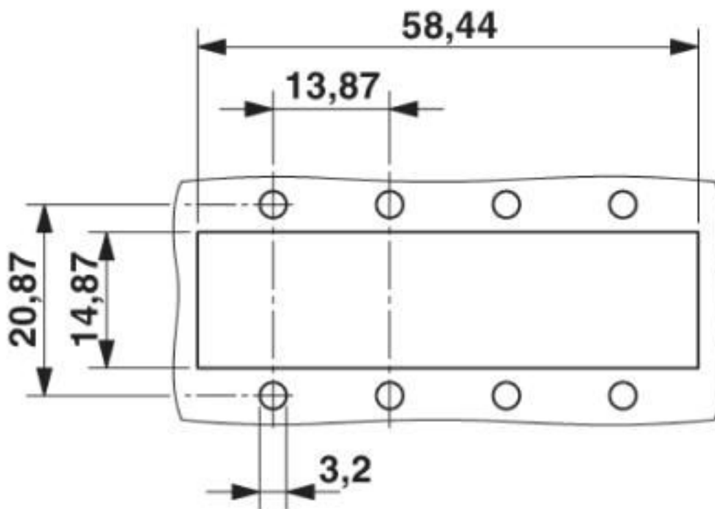
Dimensional drawing
