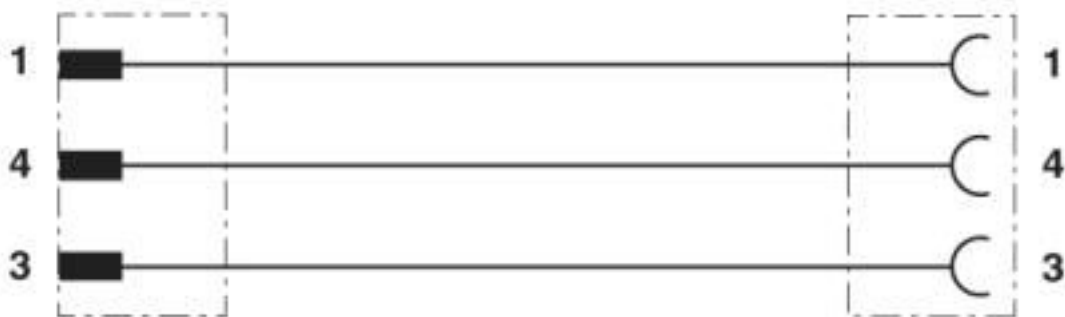
Schematic diagram
