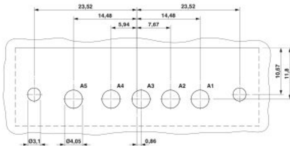
Drilling diagram
