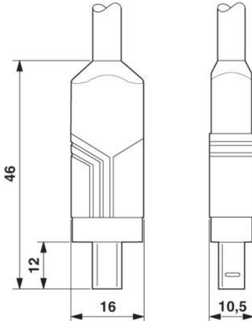
Dimensional drawing
