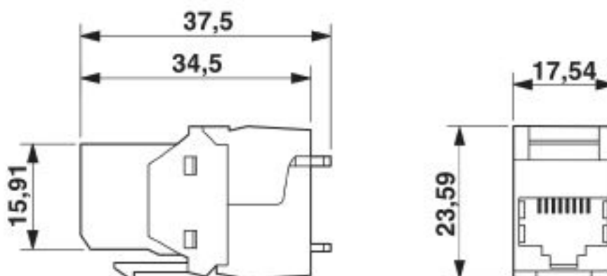
Dimensional drawing
