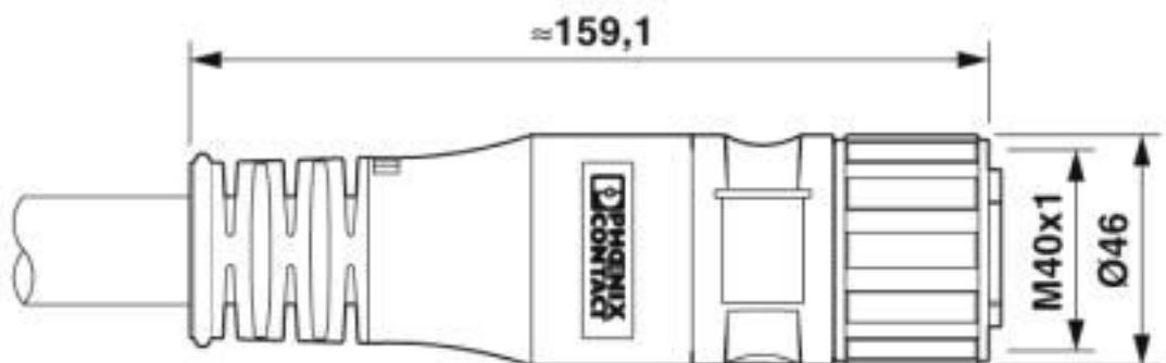
Dimensional drawing
