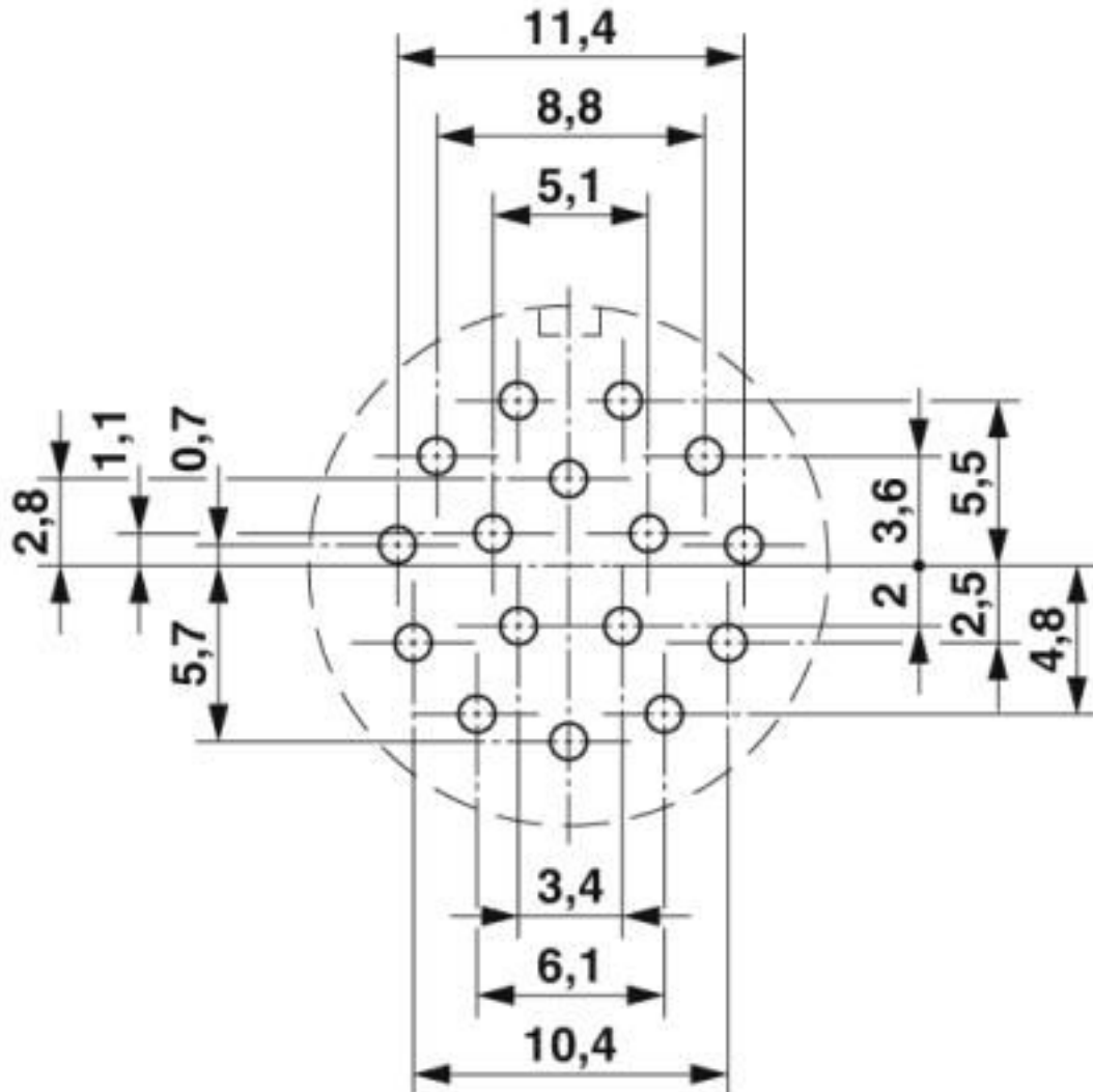
Drilling diagram
