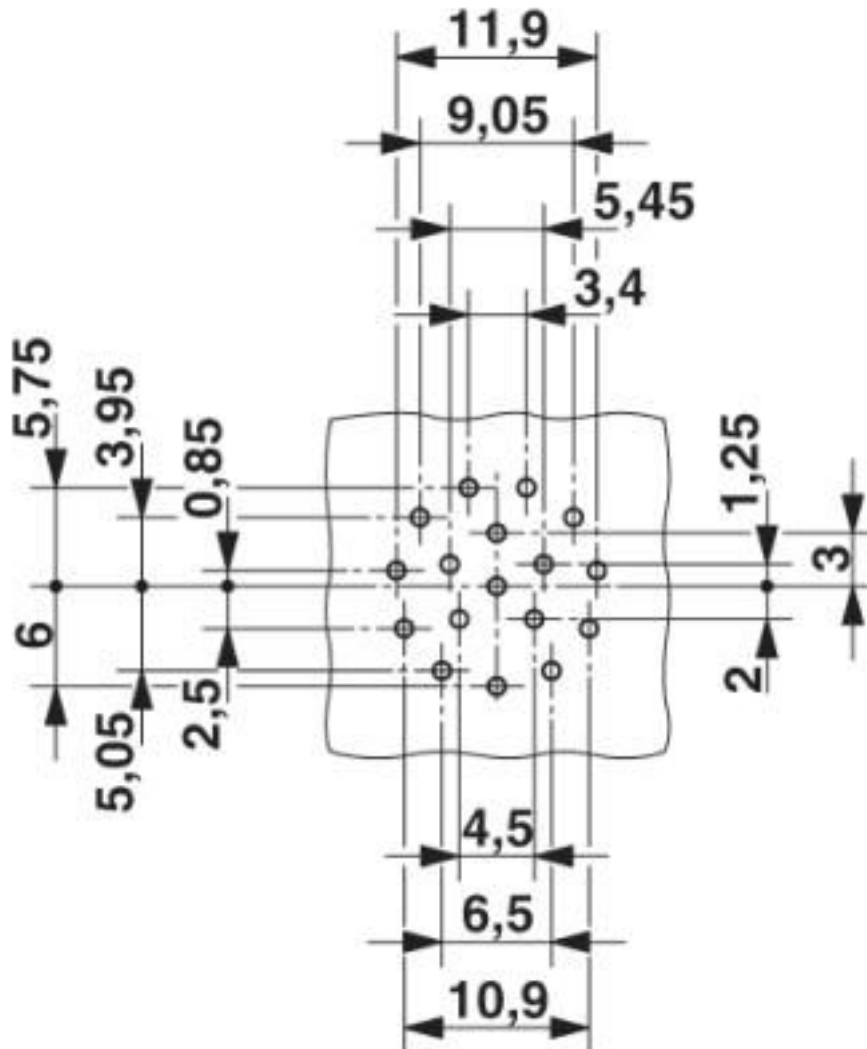
Drilling diagram
