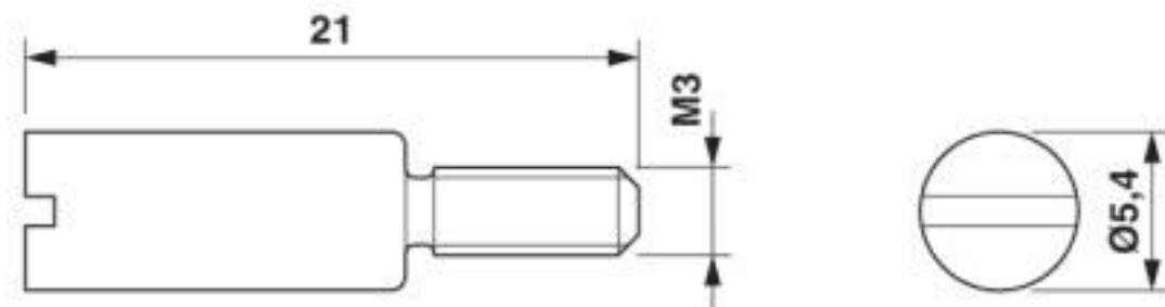
Dimensional drawing
