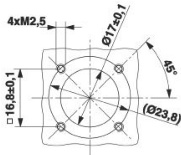
Dimensional drawing
