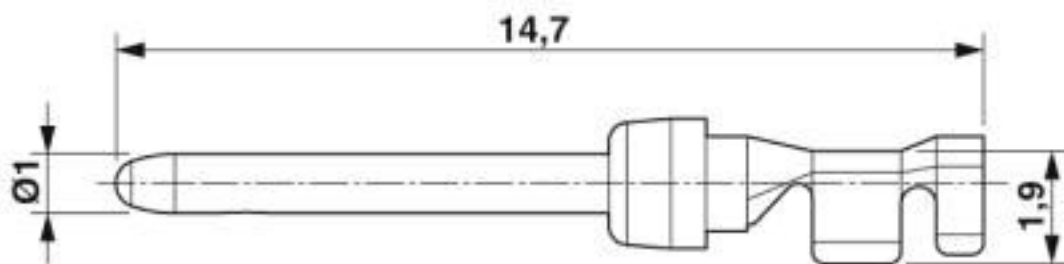
Dimensional drawing
