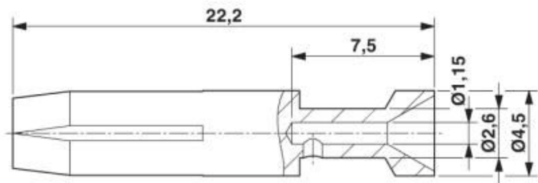
Dimensional drawing
