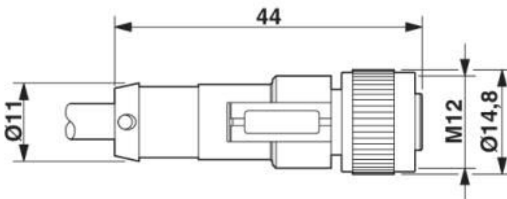
M12-SPEEDCON socket, straight
