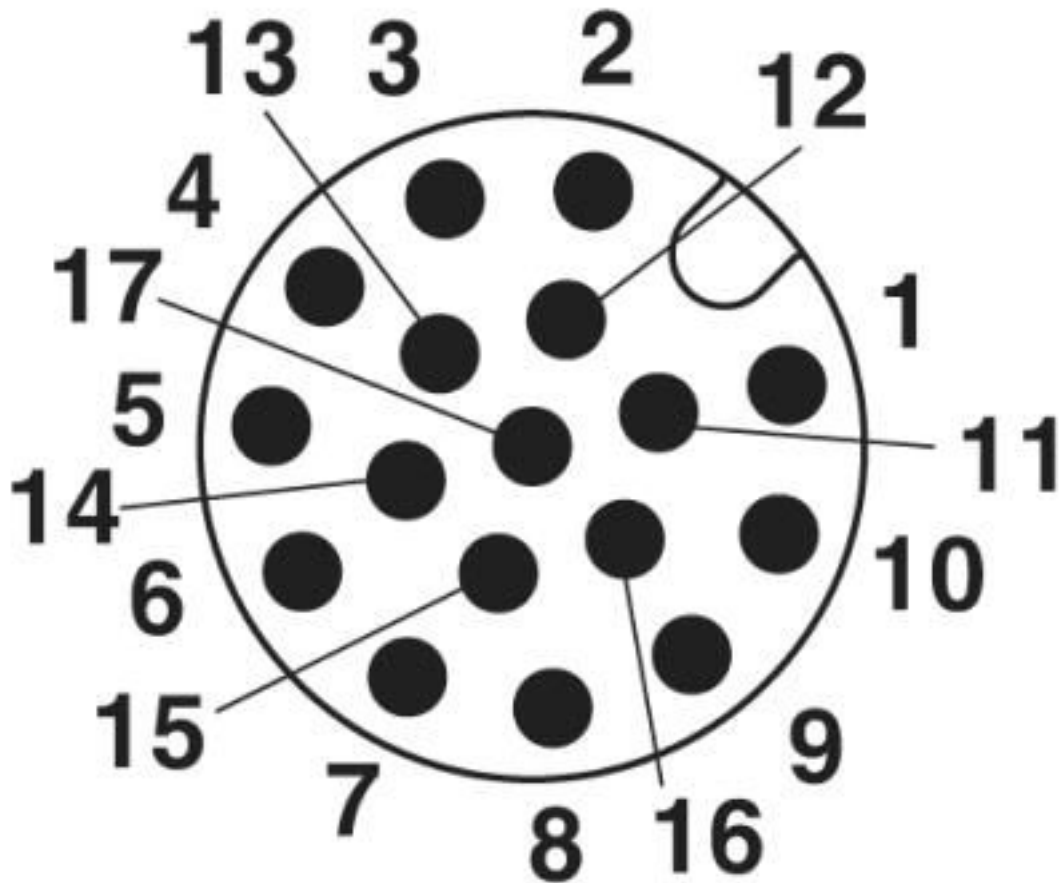
Schematic diagram
