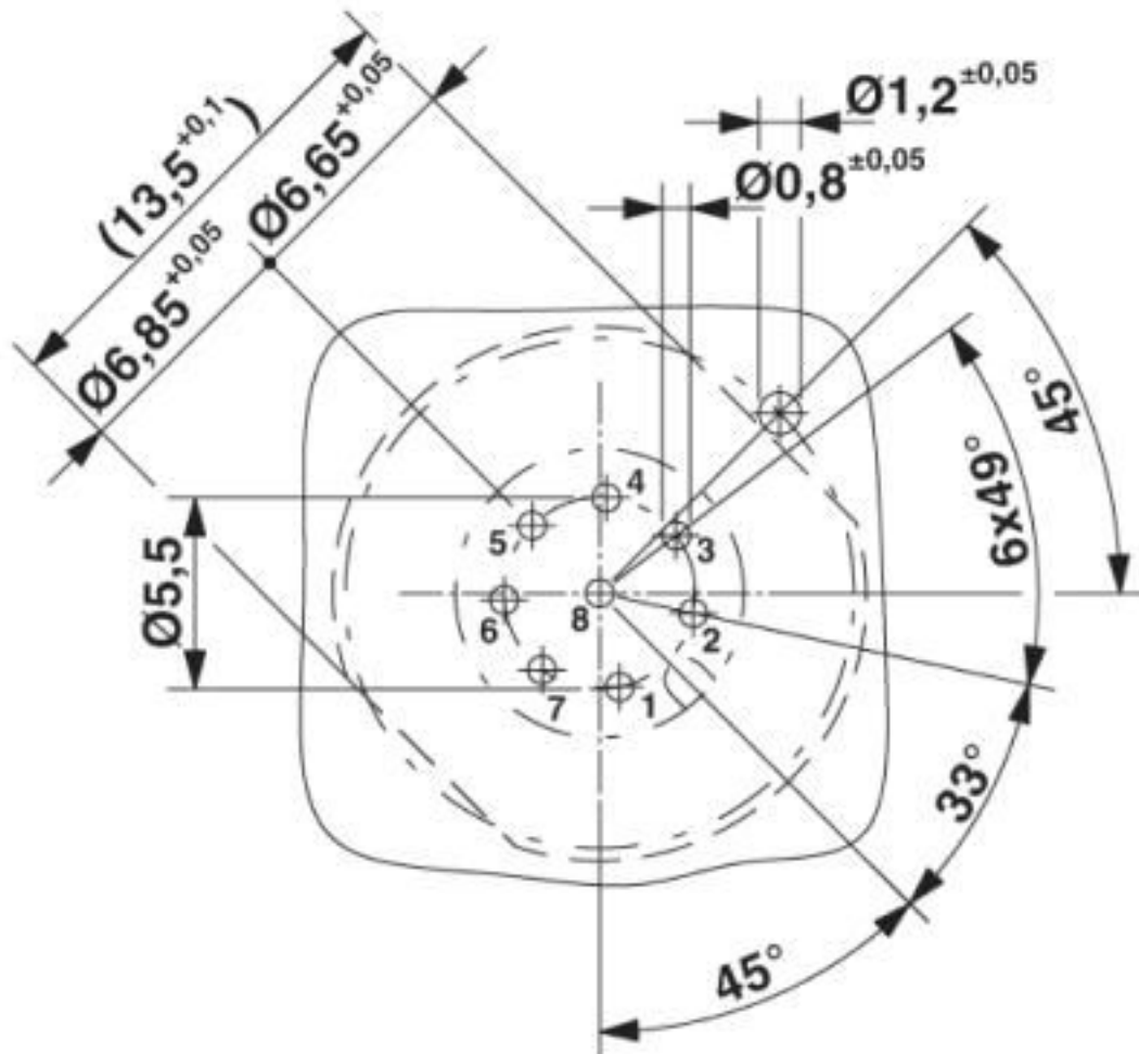
Drilling diagram
