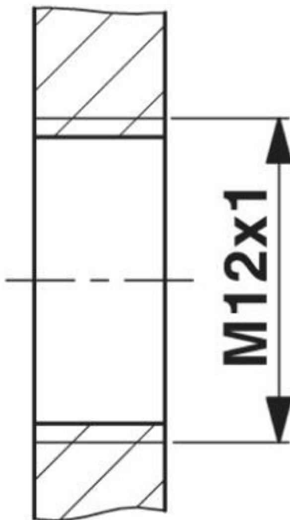
Dimensional drawing
