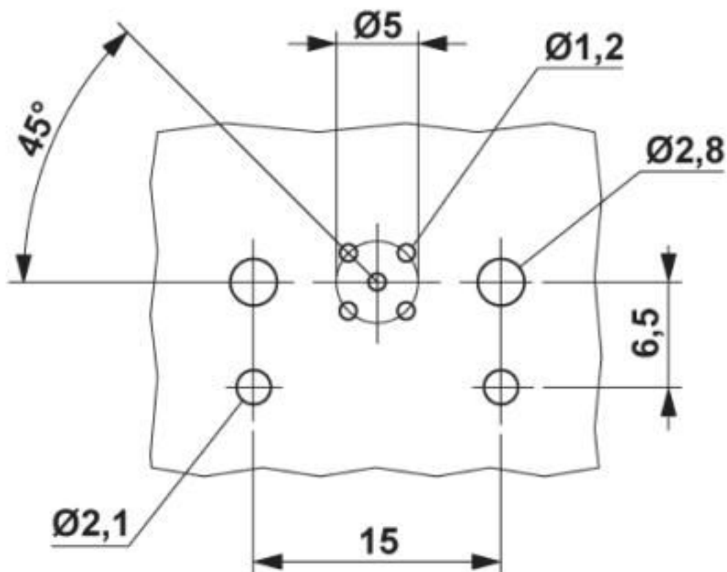
Drilling diagram
