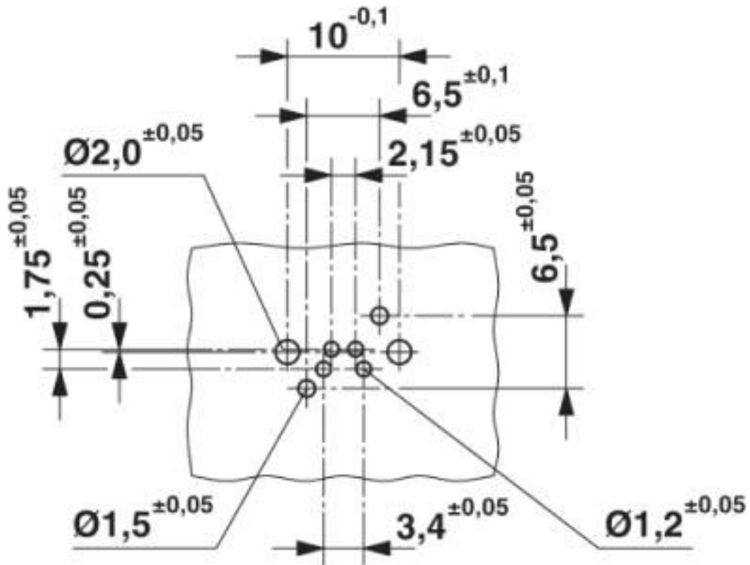
Drilling diagram
