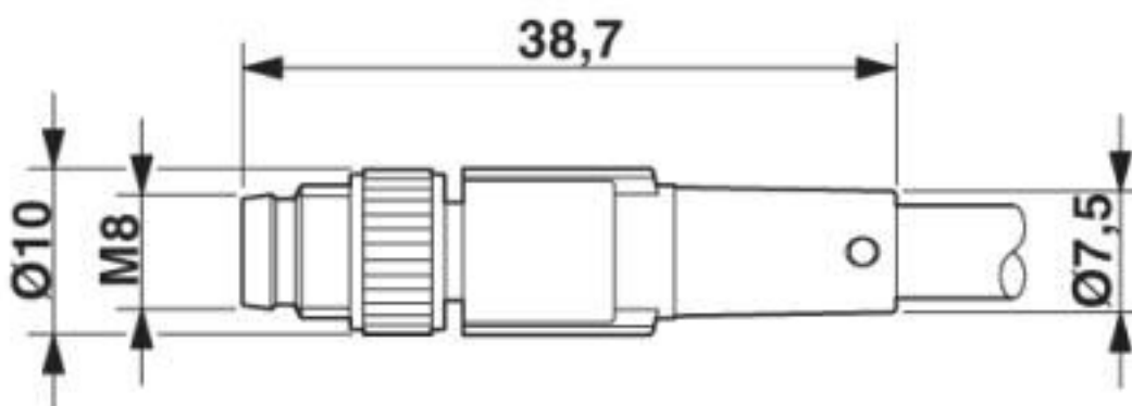
Dimensional drawing
