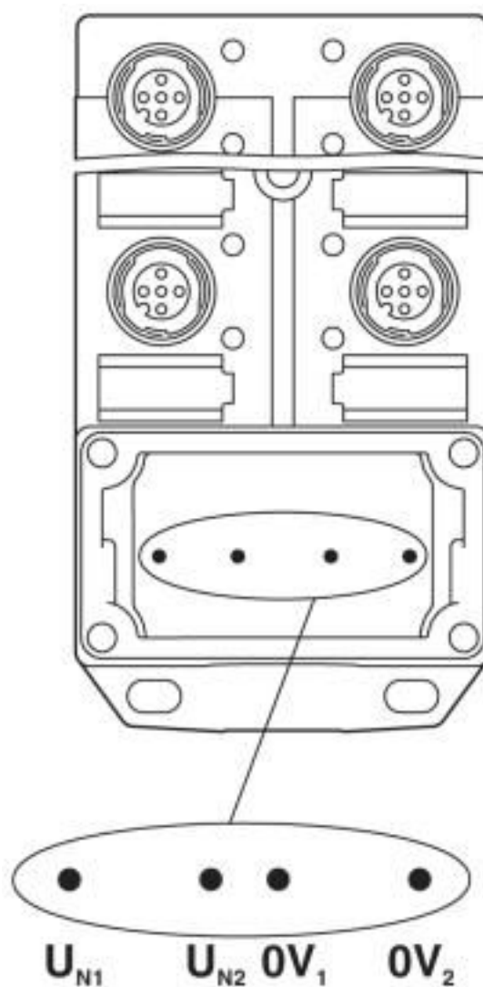
Schematic diagram
