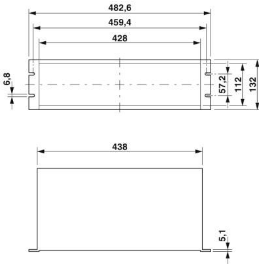
Dimensional drawing
