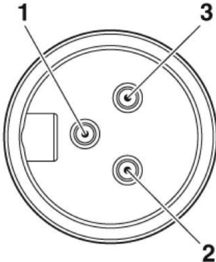
Pin assignment, plug, 7/8"-16UNF, 3-pos., view of male side
