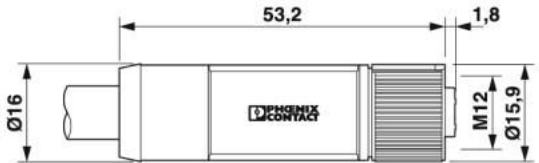
Dimensional drawing
