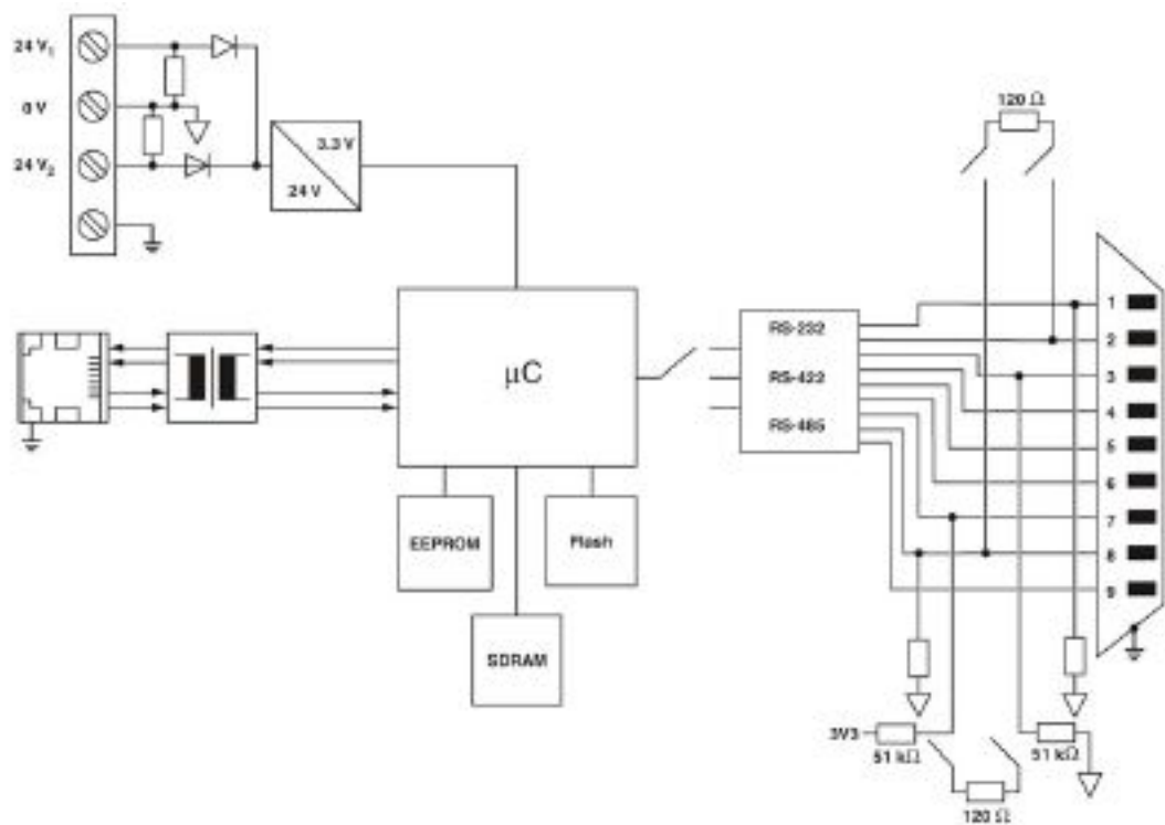
Block diagram
