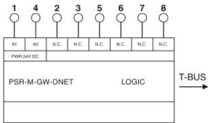
Block diagram
