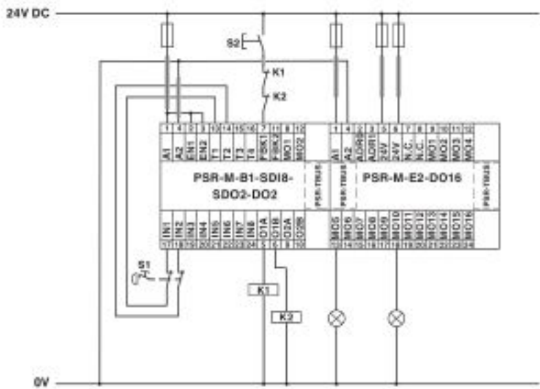
Application drawing
