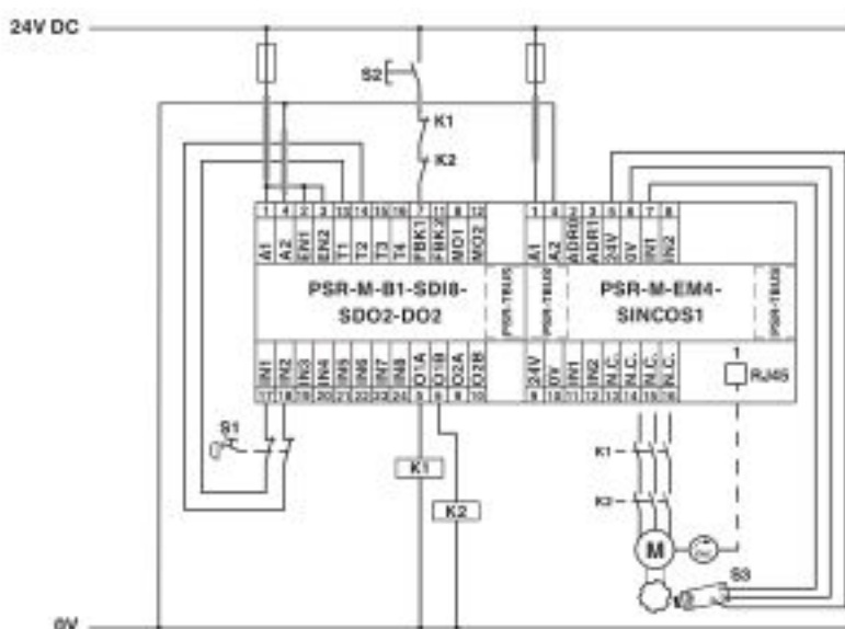
Application drawing
