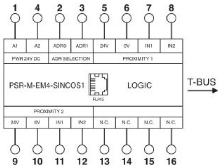
Block diagram
