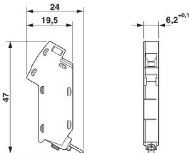
Dimensional drawing
