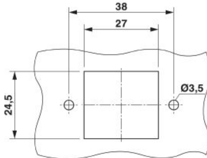
Dimensional drawing
