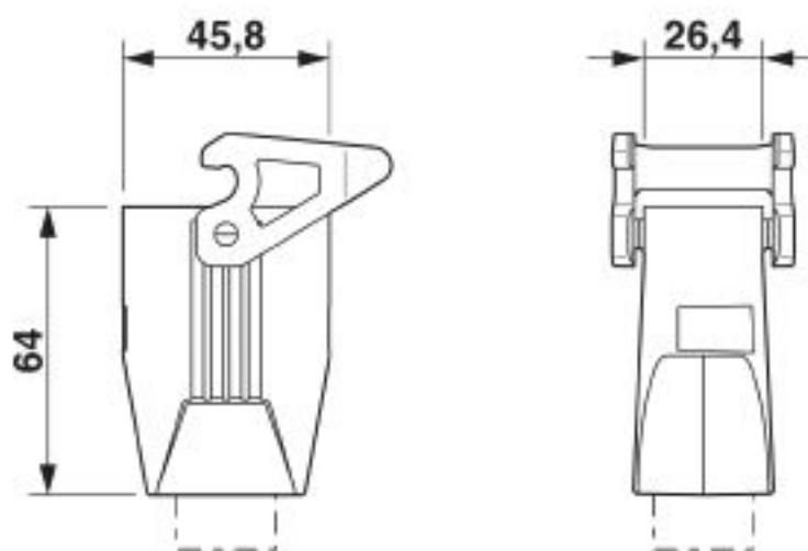
Dimensional drawing
