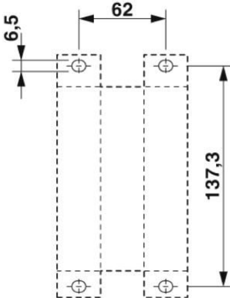
Dimensional drawing
