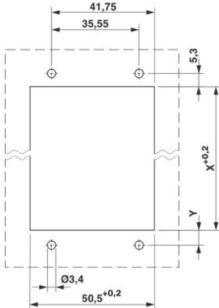
Dimensional drawing
