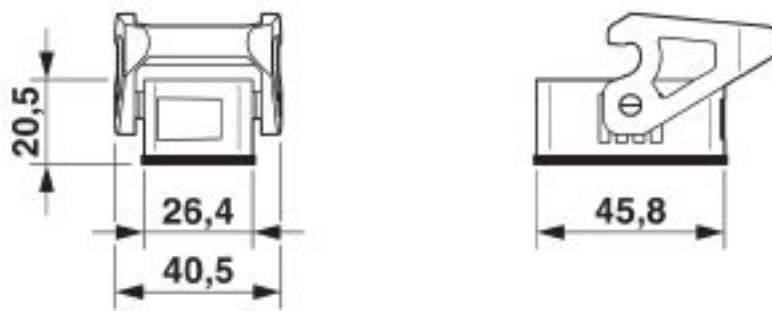
Dimensional drawing
