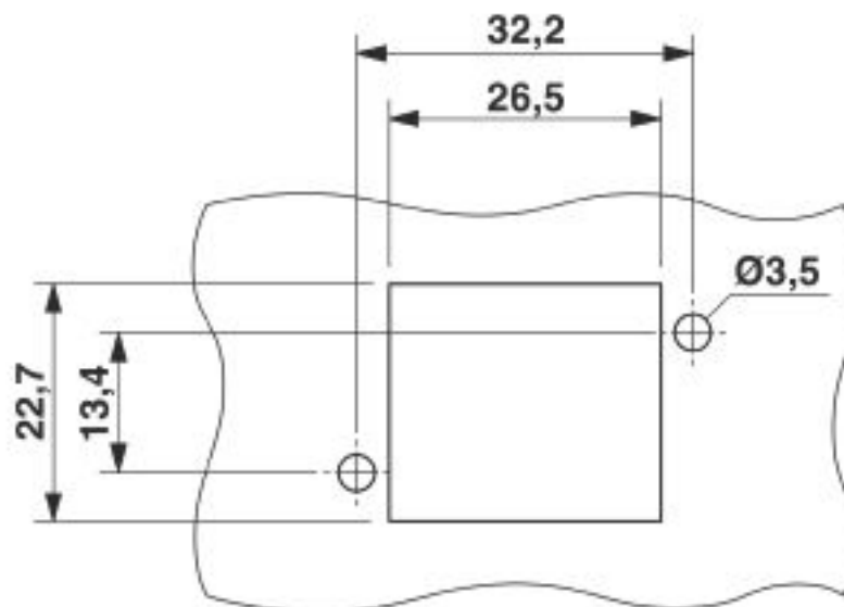
Dimensional drawing
