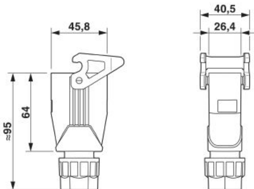
Dimensional drawing
